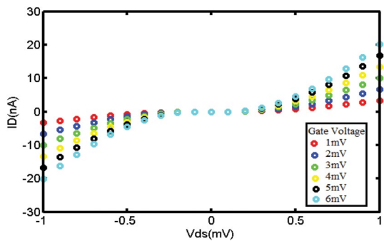
Fig. 7. Coulomb blockade ranges based on proposed model are calculated for different applied gate voltages. The applied gate voltages are 1mV, 2nm, 3mv, 4mv, 5mv and 6mv in fullerene SET.
