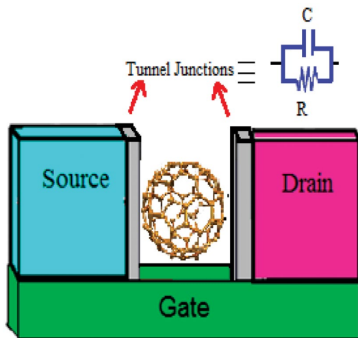
Fig. 1. Single electron transistor.
