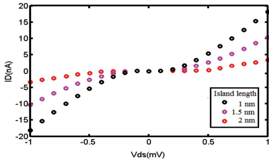
Fig. 6. coulomb blockade ranges based on proposed model are calculated. The fullerene diameters as island lengths are 1nm, 1.5nm and 2nm in SET.
