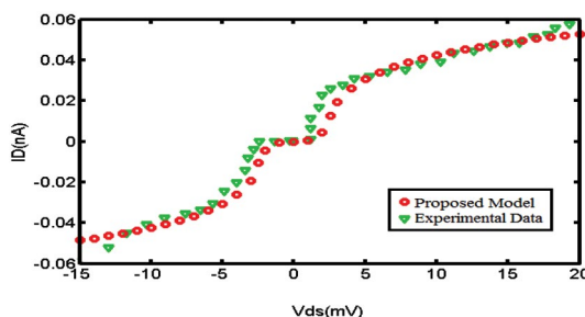
Fig. 5. comparison of current vs. voltage of fullerene SET between proposed model and experimental data that are extracted from reference [7].
