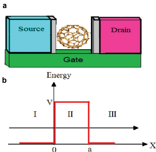
Fig. 4. (a) The SET different parts are electrodes source, drain and gate .Moreover island and two tunnel junctions are shown. (b) Island assumes a channel and SET energy vs. channel length is plotted.
