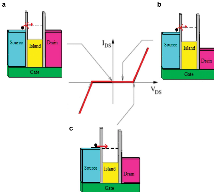
Fig. 3. I-V characteristic of SET. (a) The unequipped energy level is higher than the source Fermi level and coulomb blockade condition occurs. (b) Electrodes Fermi level is changed by applying voltage, but the unequipped energy level is higher than source Fermi level and then coulomb blockade condition occurs. (c) The source Fermi level is equal to an unequipped energy level, therefore an electron transfer to the island.
