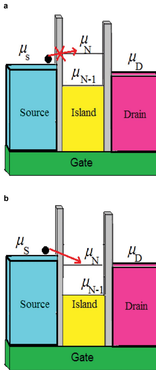
Fig. 2. (a) Coulomb blockade condition happened and the electron doesn't transfer to the island. (b) The electron tunneling occurs and the electron transfers to the island.
