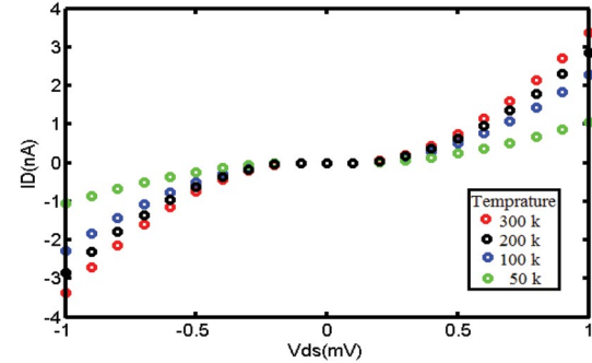
Fig. 8. Coulomb blockade ranges based on proposed model are calculated for different temperatures. The temperatures are 50k, 100k, 200k and 300k in fullerene SET.
