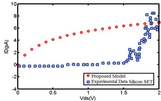
Fig. 9. The comparison current vs. drain voltage of two SETs at room temperature. The red points show the current of the fullerene SET at room temperature. The blue points show the current of silicon SET at room temperature and experimental data are extracted from reference [21].
