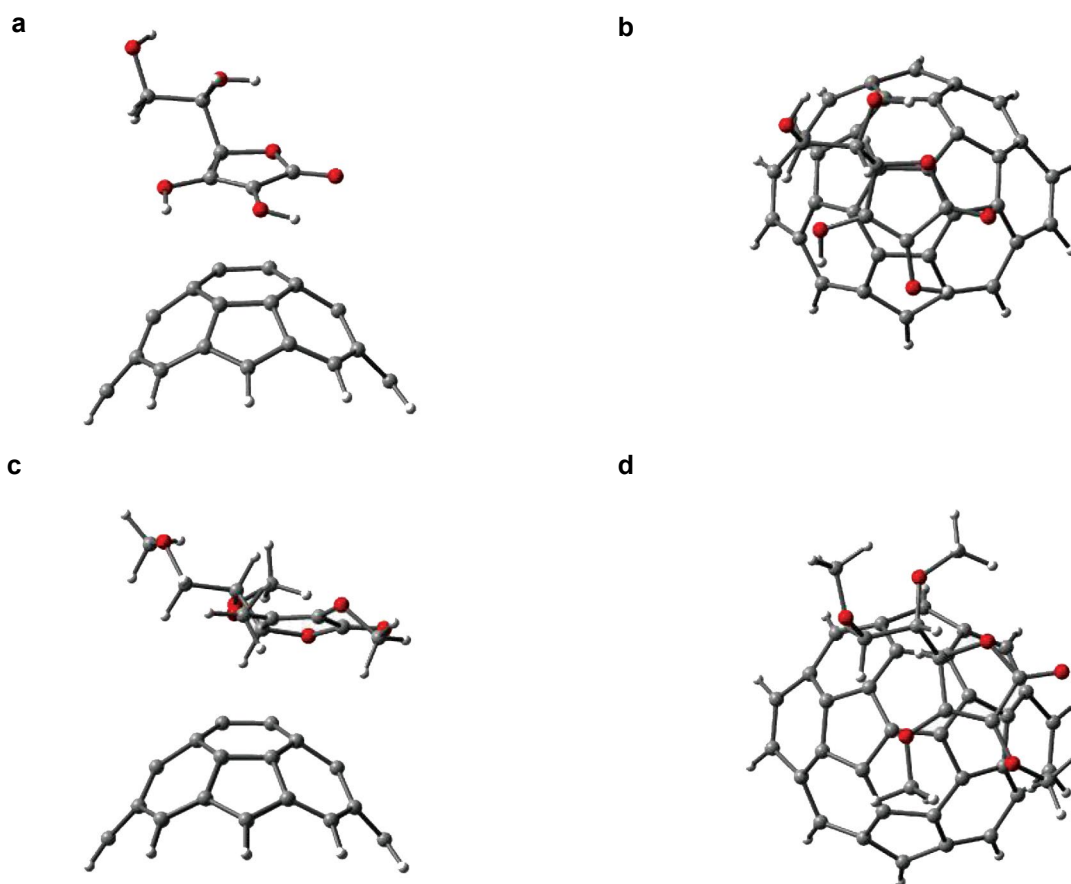
Fig. 3. (a) and (b) Different representations of OVit-Ful hybrid. (c) and (d) Different representations of MVit-Ful hybrid.
