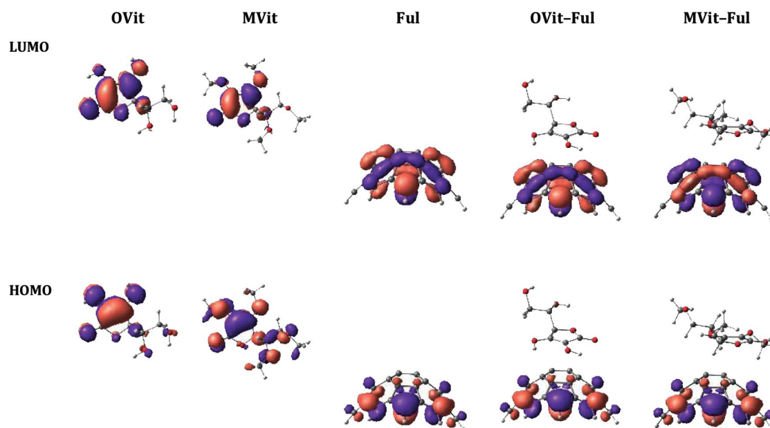
Fig. 4. HOMO and LUMO Distribution patterns. There were no significant changes between the distribution patterns in gaseous and water-solvated systems. See Figs. 1-3 for the models.
