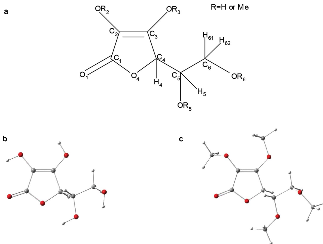
Fig. 1. (a) 2D representation of Vit (vitamin C). (b) 3D representation of OVit (original Vit). (c) 3D representation of MVit (methylated Vit).
