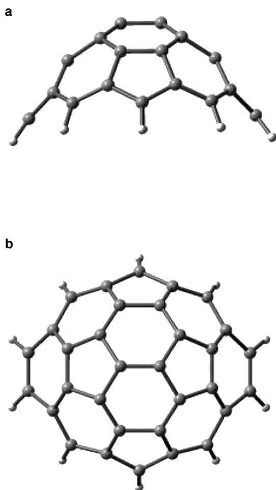
Fig. 2. Side and Up views of Ful (fullerene surface).
